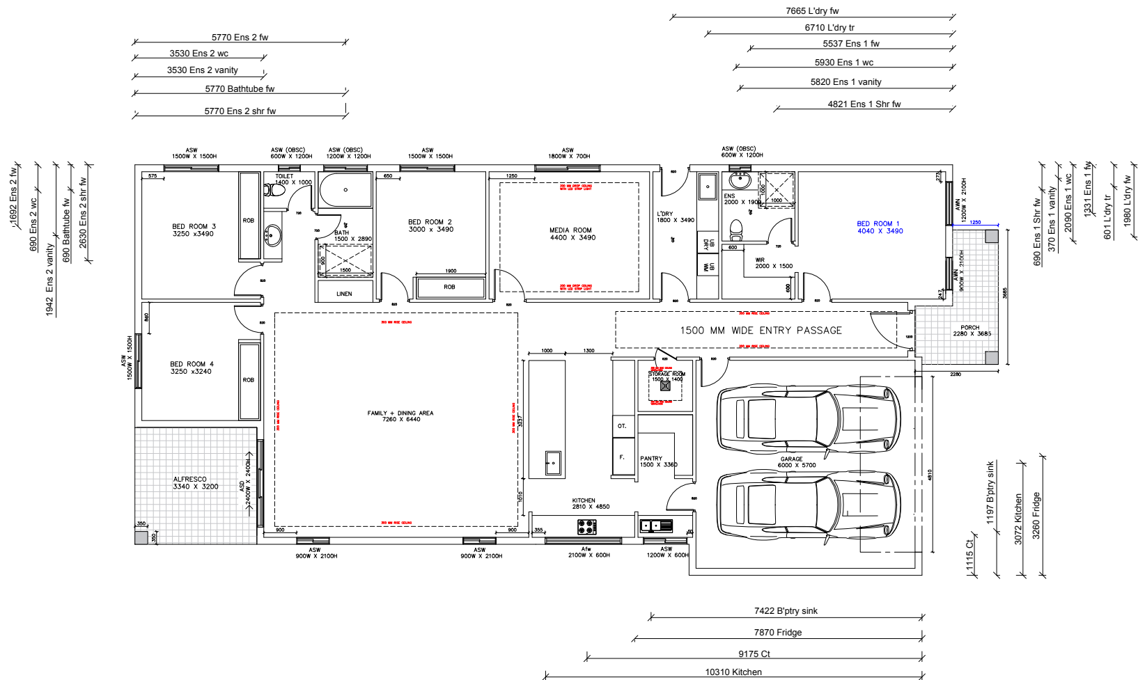
PLUMBING LAYOUT SCALE 1:100
